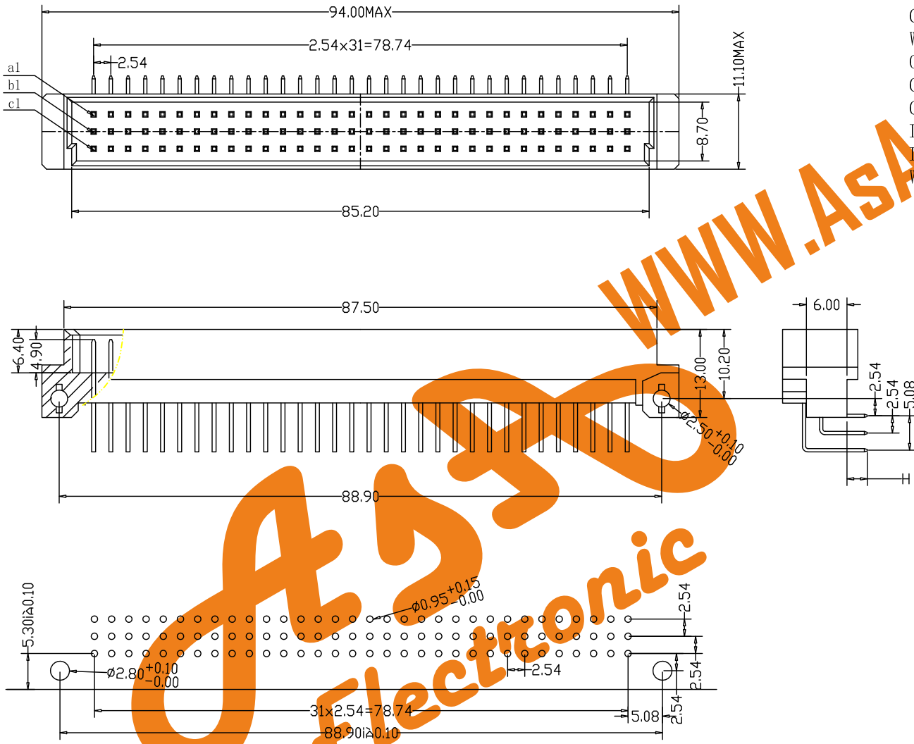
Recommended P.C.B.Layout
